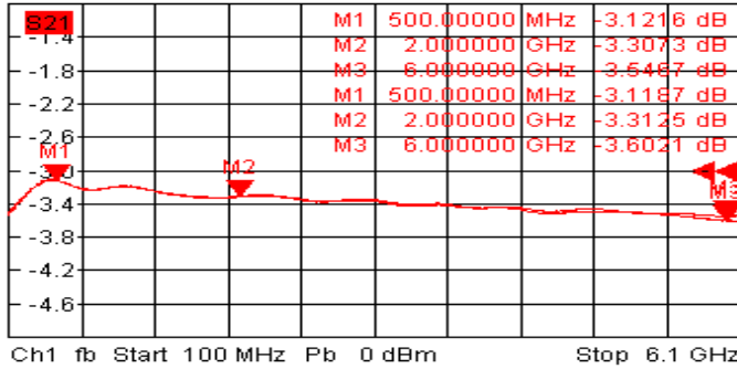
Trc3 S21 dB Mag 0.4 dB / Ref -3 dB Cal 3
