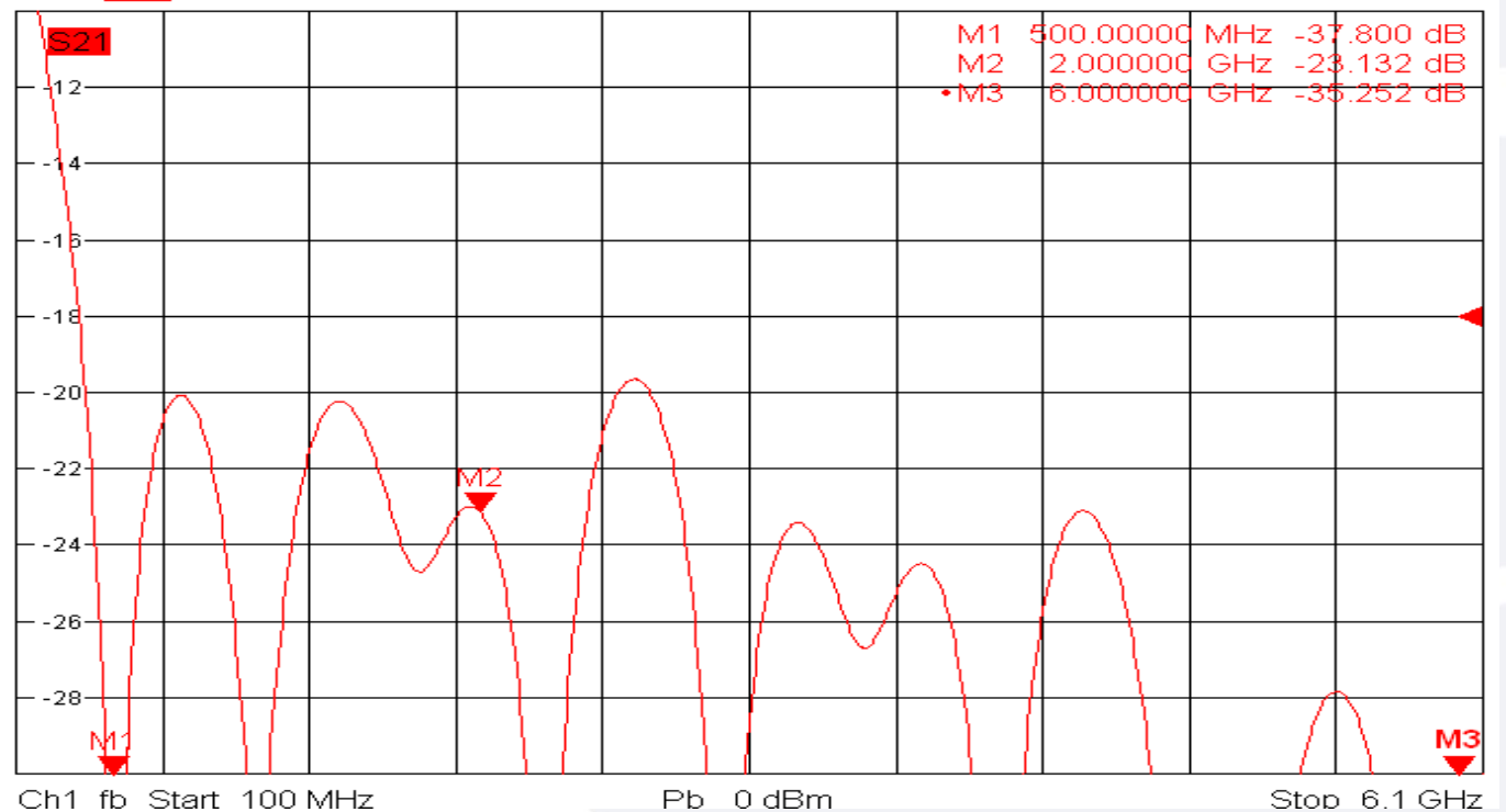
Trc1 S21 dB Mag 2 dB / Ref -18 dB Cal 1
