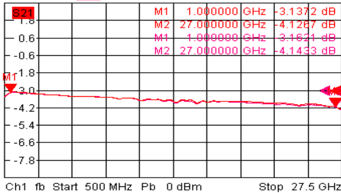
Trc3 S21 dB Mag 1.2 dB / Ref-3 dB Cal 3 Mem6[Trc3] S21 dB Mag 1.2 dB / Ref-3 dB
