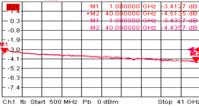
Trc3 S21 dB Mag 1.1 dB / Ref -3 dB Cal 3 Mem6[Trc3] S21 dB Mag 1.1 dB / Ref -3 dB
