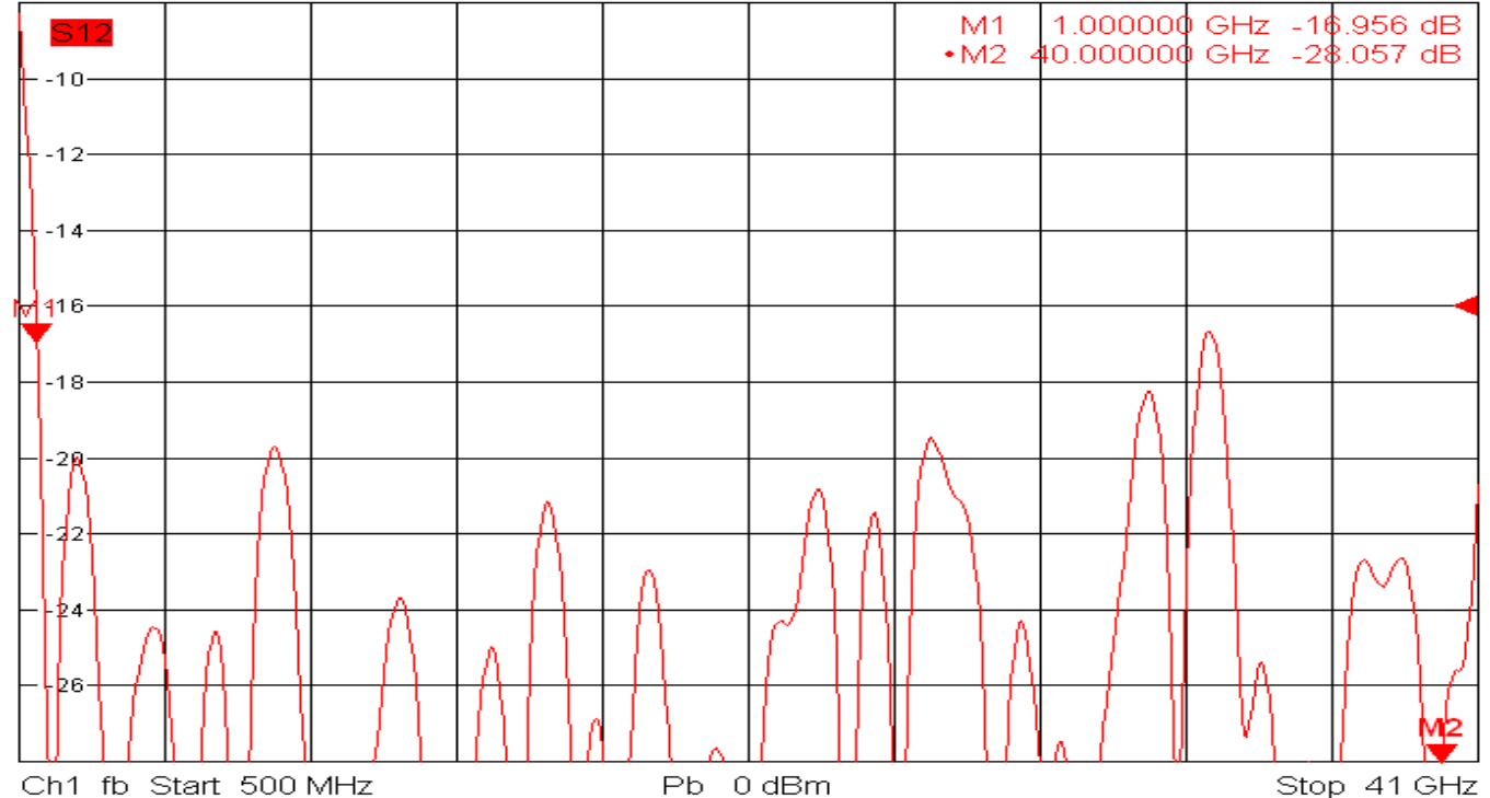
Trc2 S12 dB Mag 2 dB / Ref -16 dB Cal 2 (Max)
