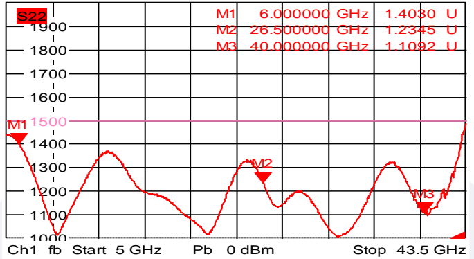
Trc4 S22 SWR 100 mU/ Ref 1 U Cal 4
