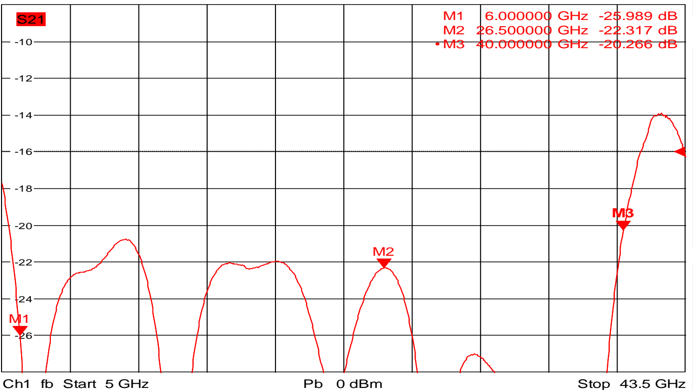
Trc2 S21 dB Mag 2 dB / Ref -16 dB Cal
