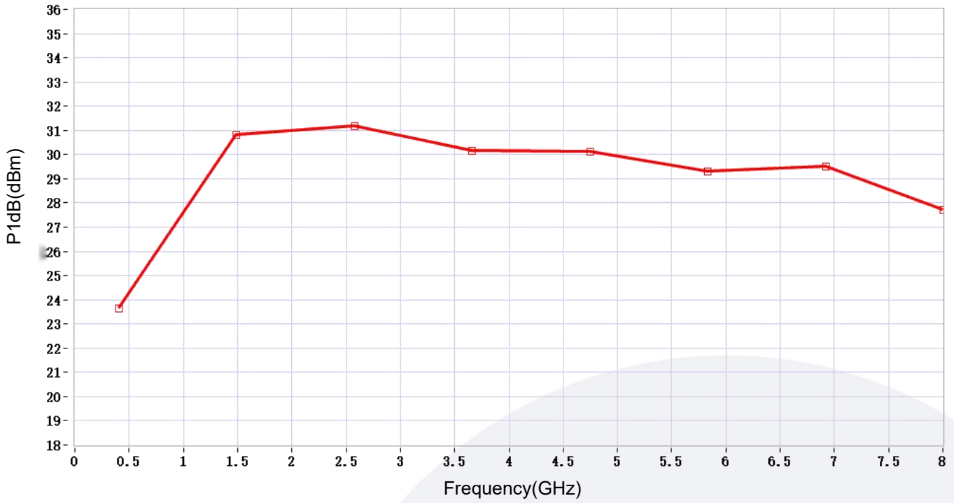
P1dB vs Frequency
