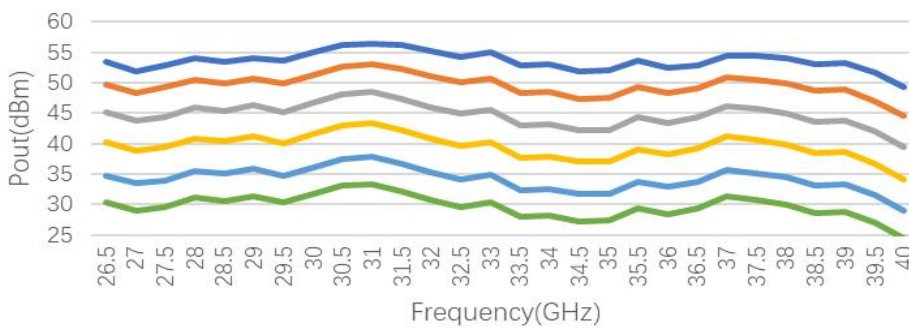
Pout@Equal-Pin
