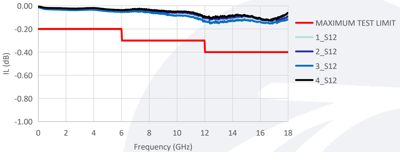
INSERTION LOSS
