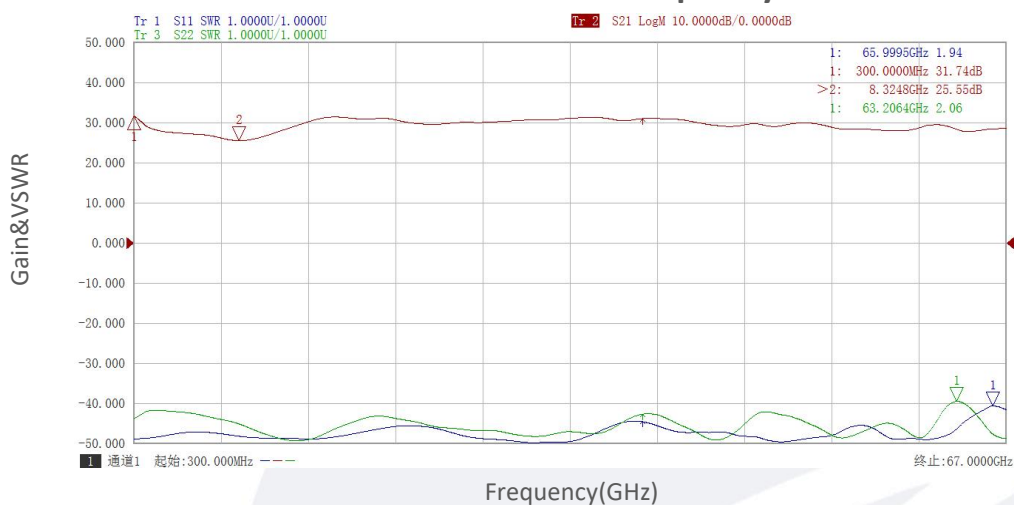
Gain&VSWR vs Frequency
