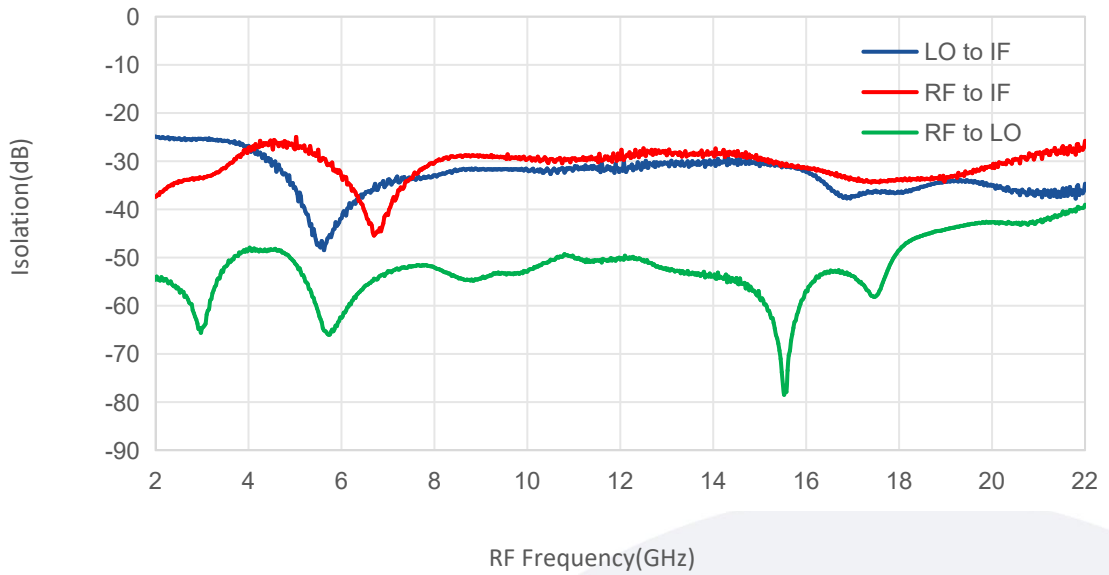
Isolation vs RF Frequency
