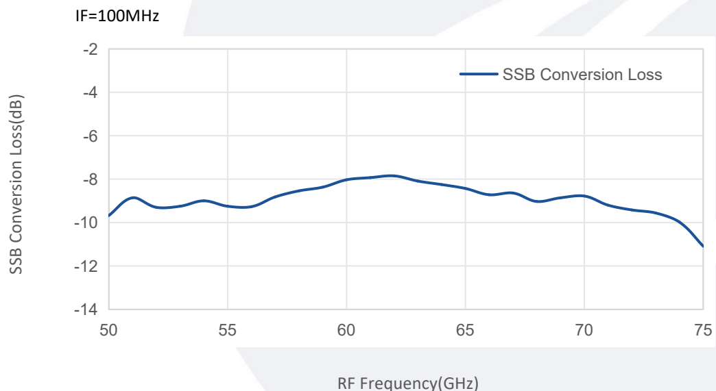
SSB Coverison Loss vs RF Frequency
