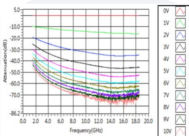
Attenuation vs Frequency
