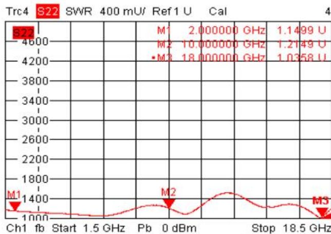
Output VSWR vs Frequency
