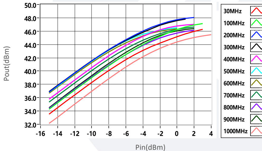
Pout vs Pin
