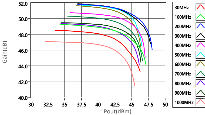
PndB vs Frequency
