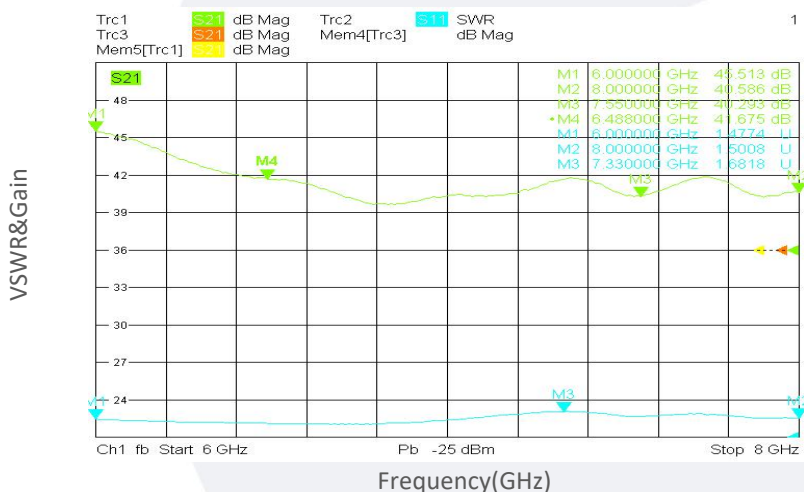
VSWR&Gain vs Frequency
