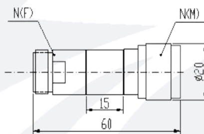
Connector: N and TNC are optional. Unit : mm
