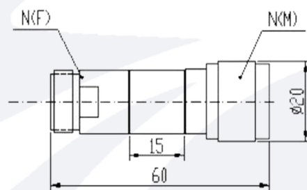
Connector: N and TNC are optional. Unit : mm
