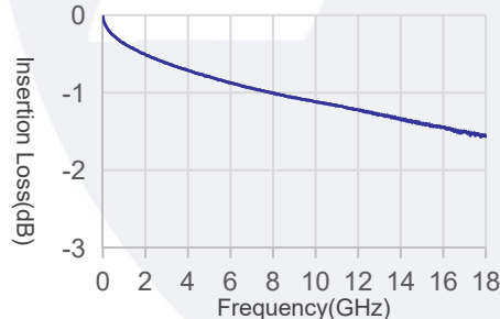
A40-SMAMSMAWM-1m INSERTION LOSS
