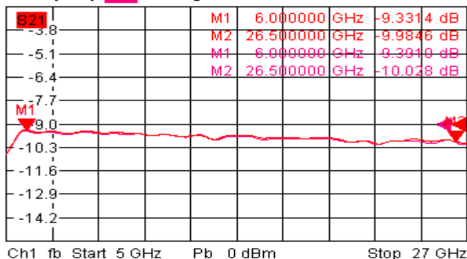
Trc3 S21 dB Mag 1.3 dB / Ref-9 dB Cal 3 Mem6[Trc3] S21 dB Mag 1.3 dB / Ref-9 dB
