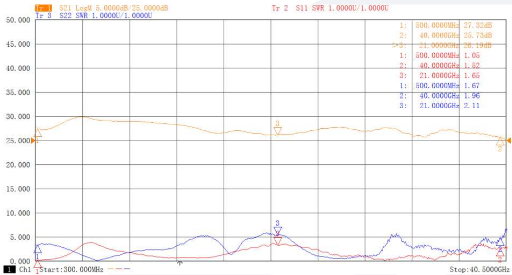
Gain&VSWR VS. Frequency
