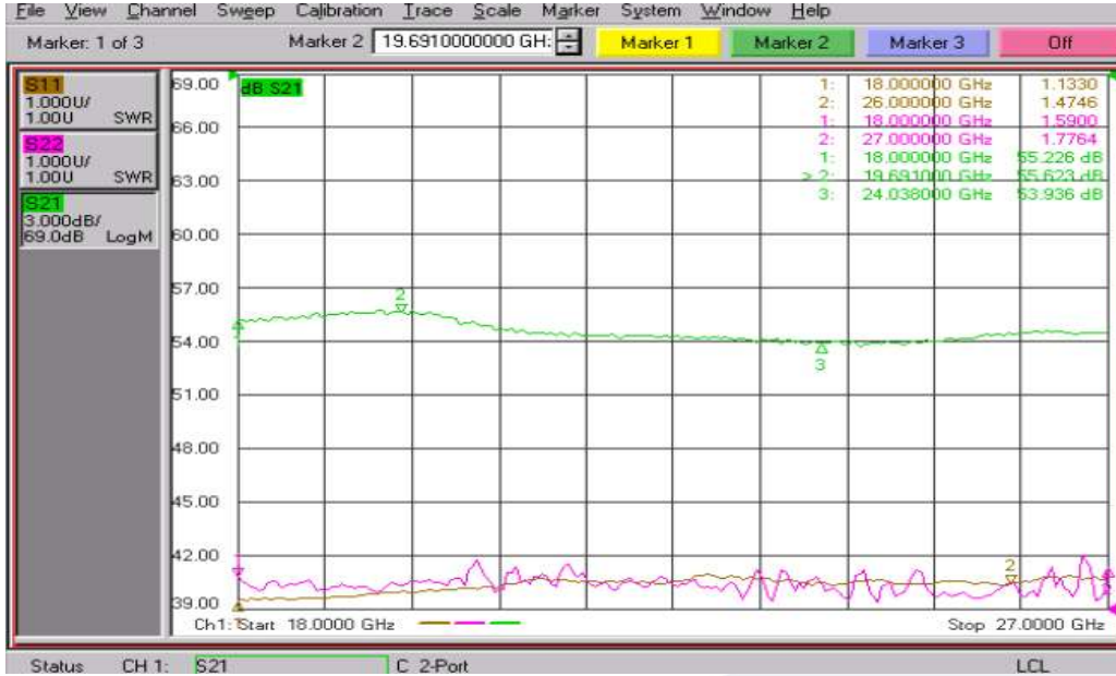
Gain&VSWR VS. Frequency
