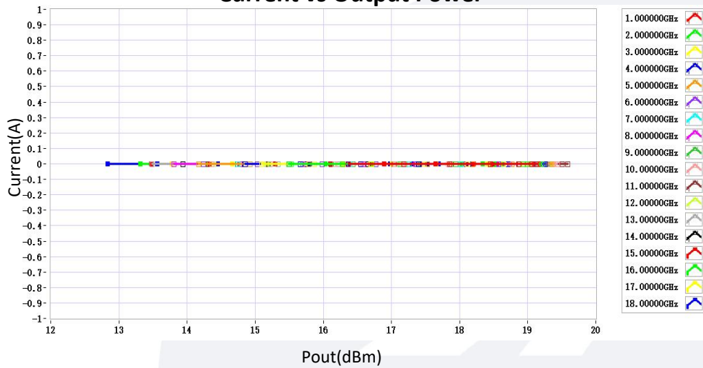
Current vs Output Power
