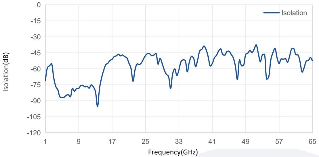
DC to Com Isolation vs Frequency
