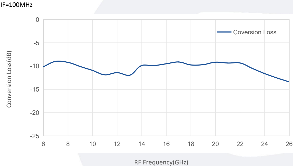
Coverison Loss vs RF Frequency
