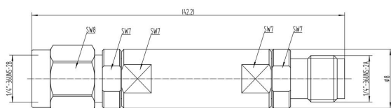
TLME-DC20G-10
