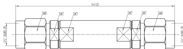
TLME-DC20G-10-MM
