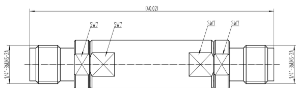
TLME-DC20G-10-FF
