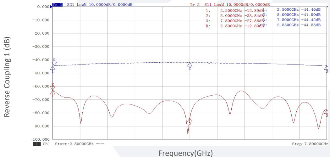
Reverse Coupling 1 vs Frequency
