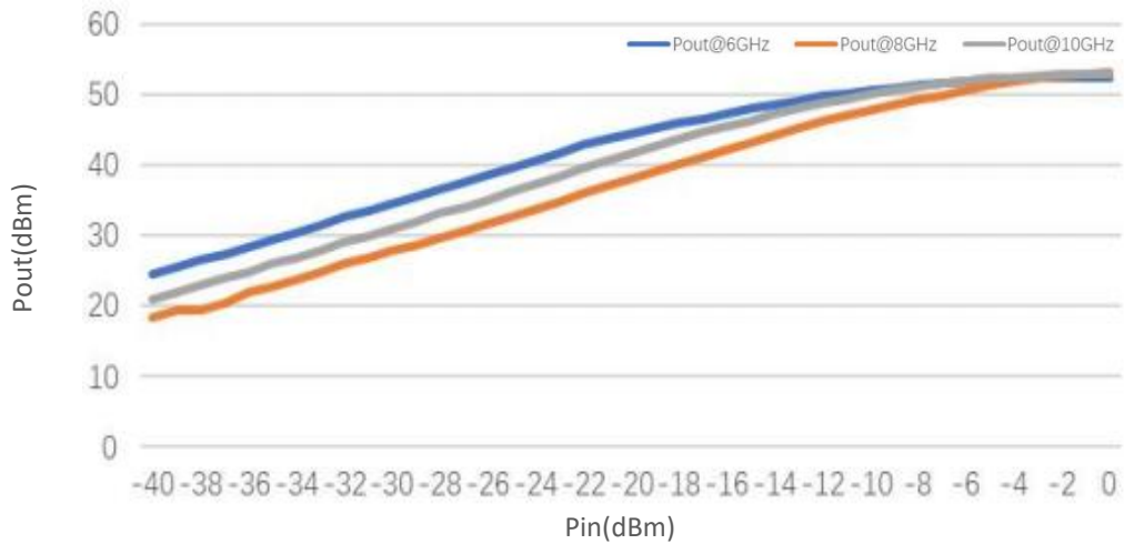
Pout@Equal_Pin
