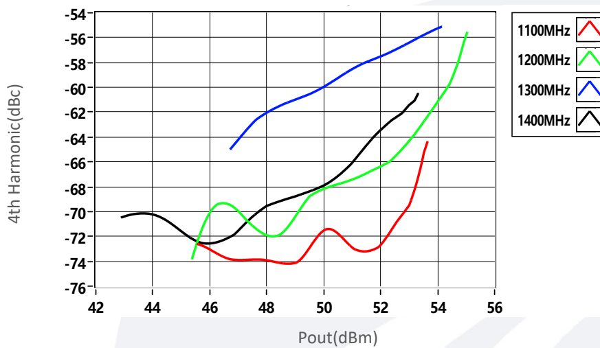
4th Harmonic vs Output Power
