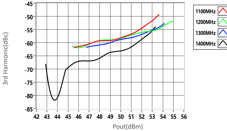
3rd Harmonic vs Output Power
