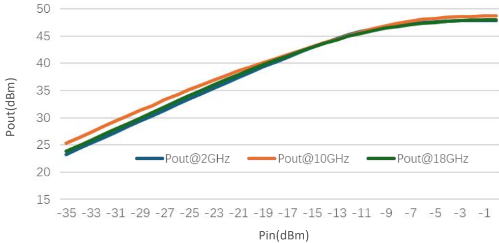
Pout@Equal_Pin
