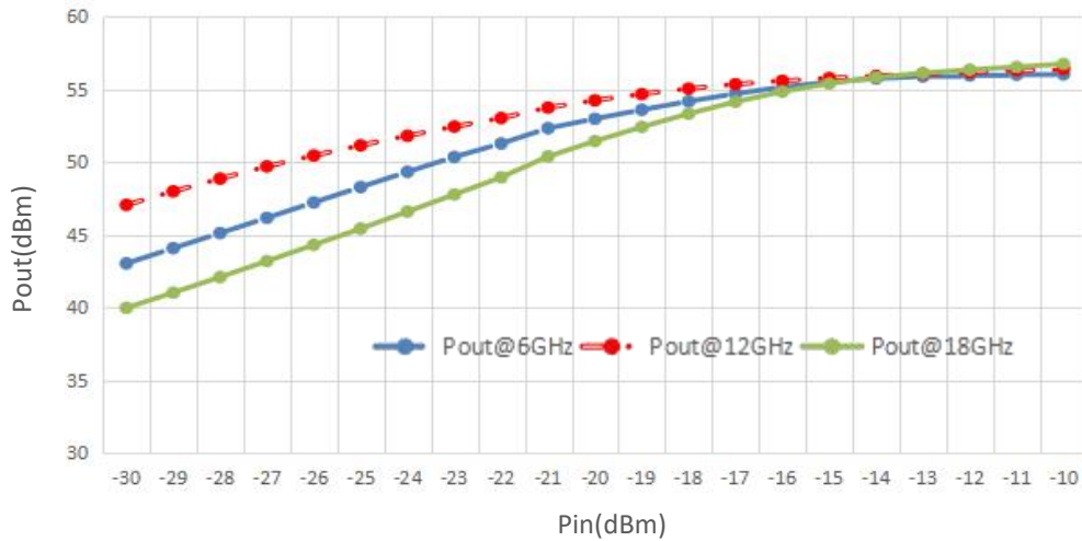
Pout@Equal_Pin
