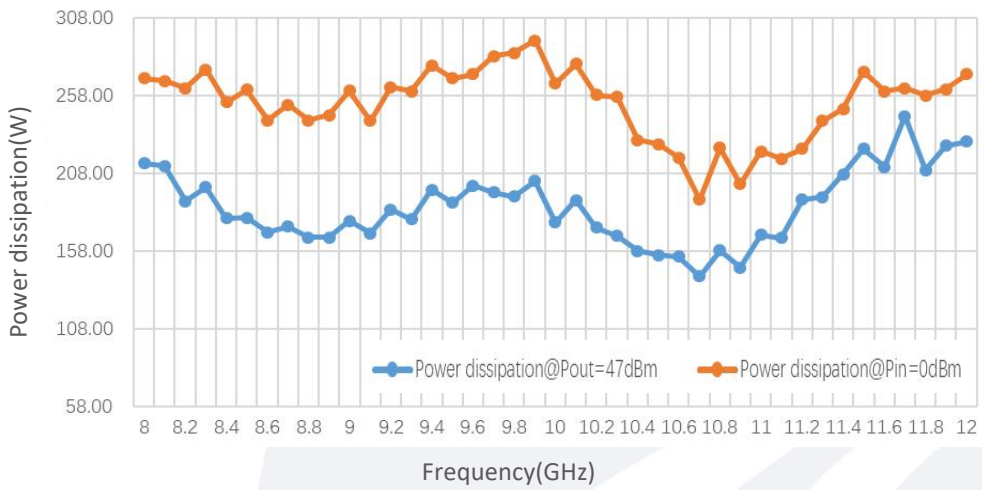
Power dissipation
