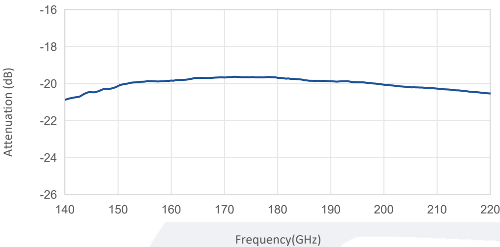
Attenuation vs Frequency
